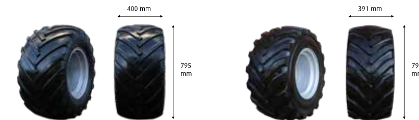
Trelleborg 400/50-15 T463
